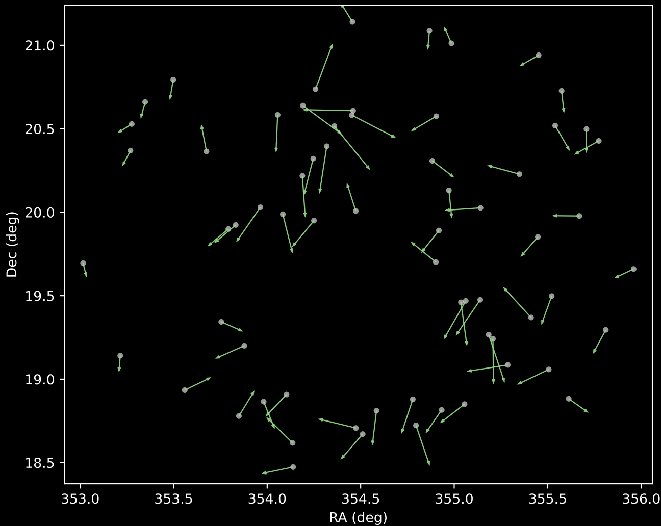
APOGEE DR17 Cluster 5 Proper Motion Vectors (n=66)
