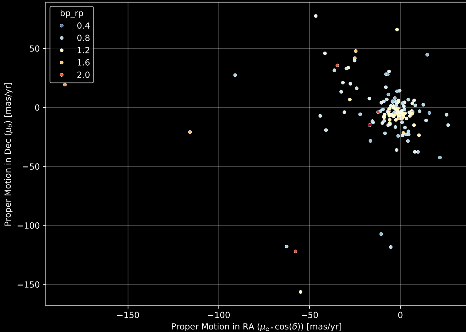
APOGEE DR17 Field: [040+34_MGA] Proper Motion Diagram (n= 146)
