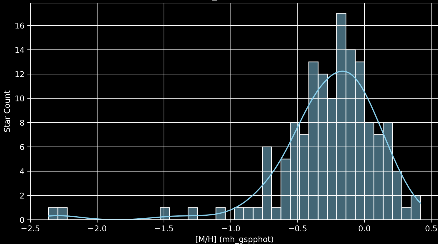
APOGEE DR17 Field: [040+34_MGA [M/H] (mh_gspphot) (n= 144)
