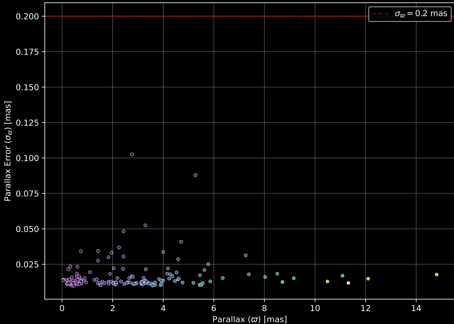
APOGEE DR17 Field: [040+34_MGA] Parallax Quality (n= 146)
