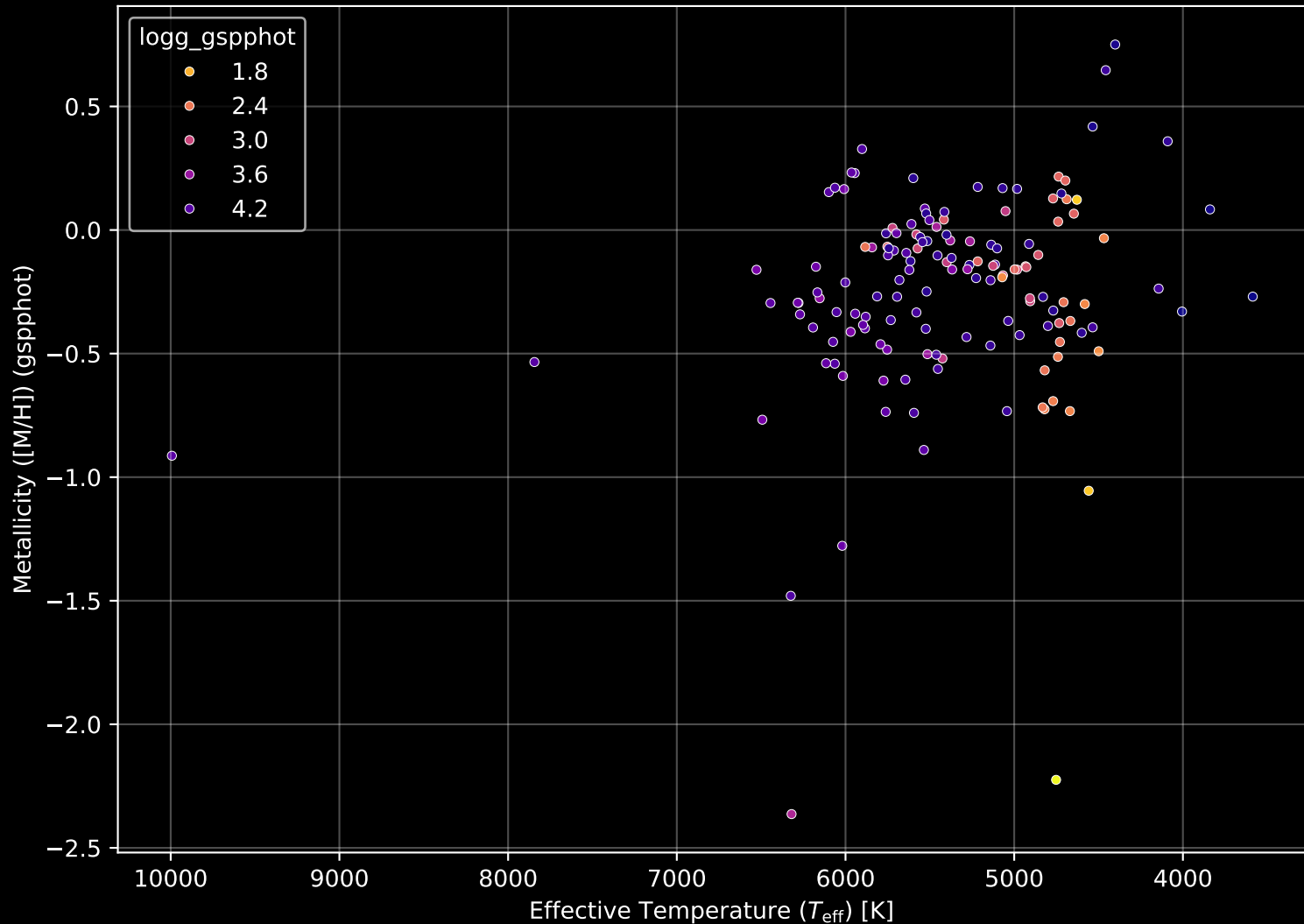
APOGEE DR17 Field: [040+34_MGA] Stellar Population Parameters (n= 146)
