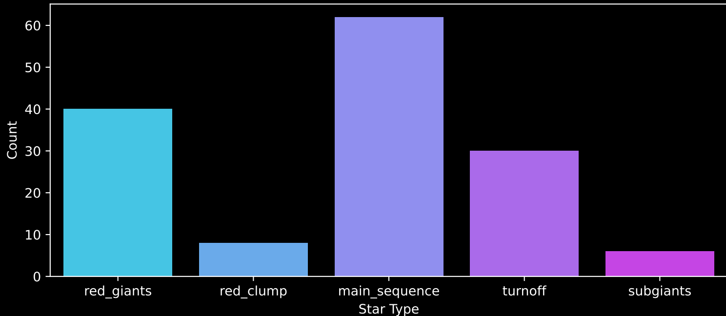
APOGEE DR17 Field: [040+34_MGA] Count plot of Star Type
