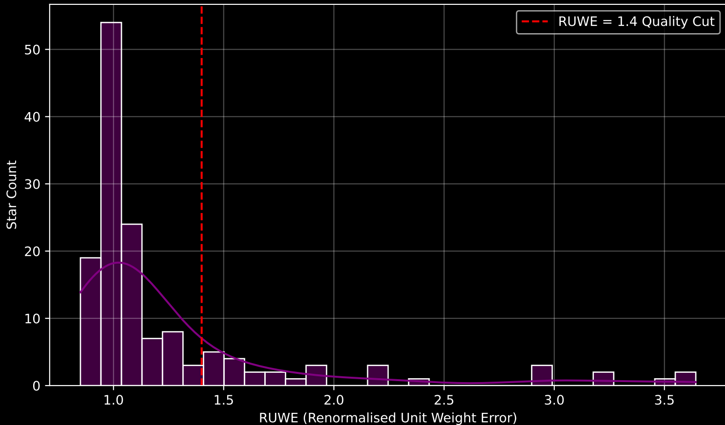
GAPOGEE DR17 Field [040+34_MGA] RUWE Distribution (n= 144)
